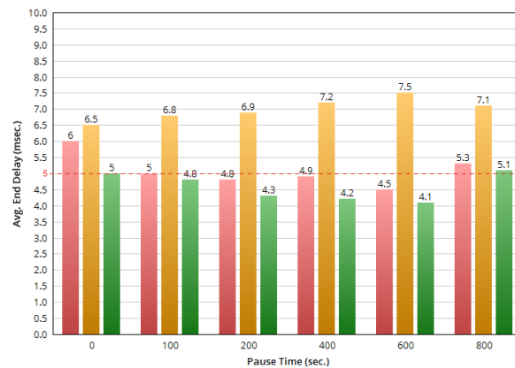
Fig.4.2: - Analysis of End-to-End Delay
