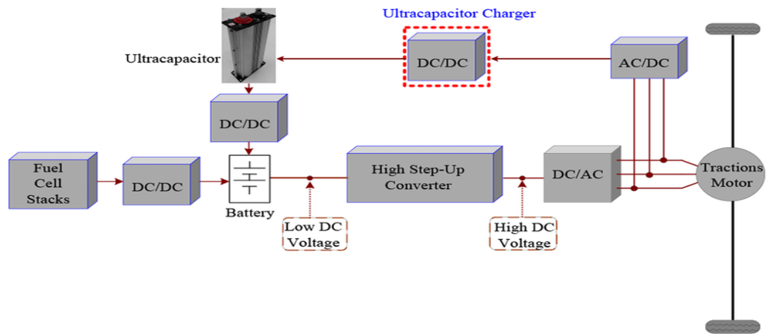
Figure 2. Basic diagram of Hybrid energy storage systems
