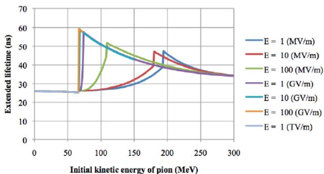
Figure 4: Lifetime extension of pions by each external electric field after 2 m drift space.
